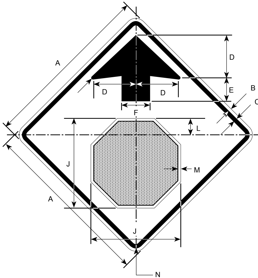
DIMENSIONS (MILLIMETERS)
