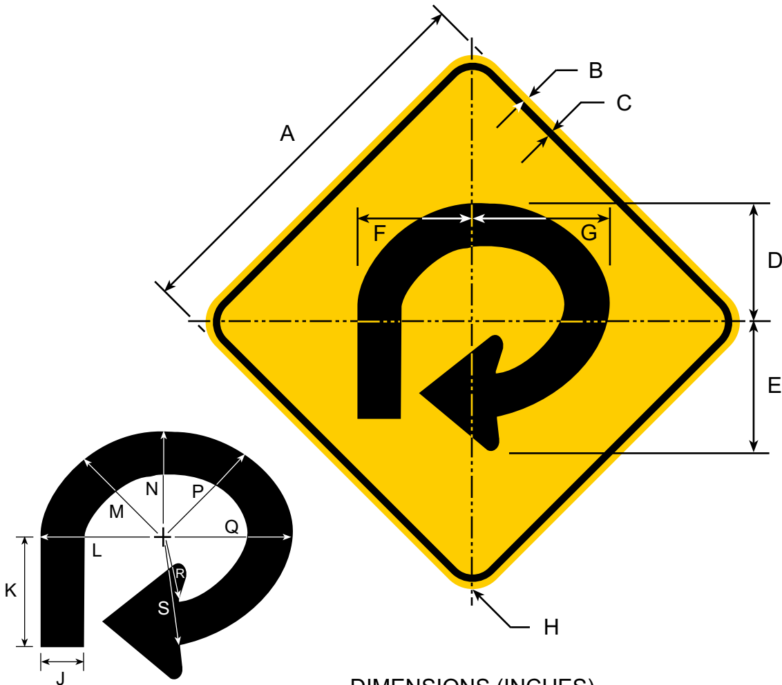
DIMENSIONS (INCHES)
