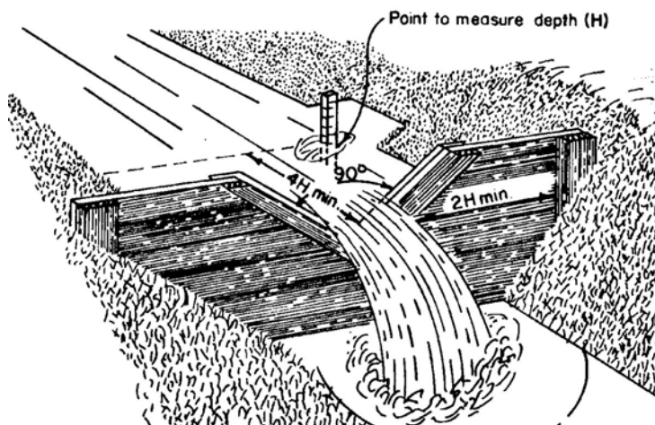
V-notch Weir
