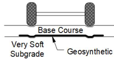
S. Geosynthetic Subgrade Reinforcement for Temporary Roads
