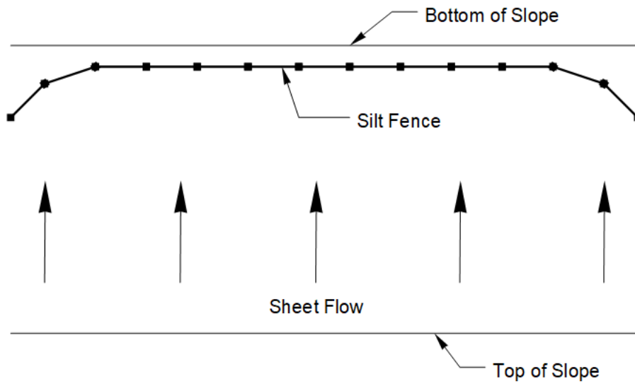
Silt Fence Plan
